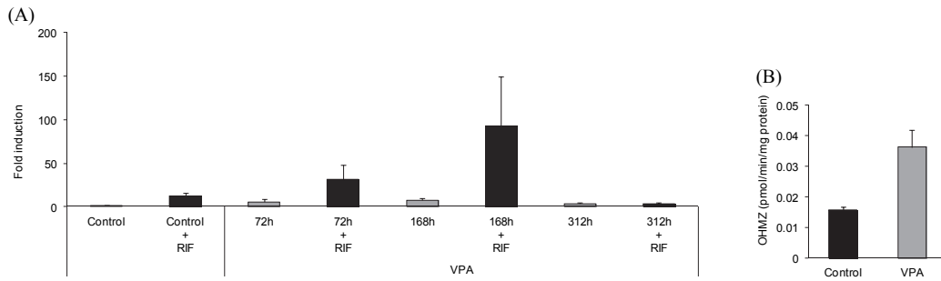
Fig. 2. Effect of RIF on CYP3A4 mRNA expression (A) and CYP3A4/5 activity (B) (A) VPA was treated for 72 hours from day 18 (72h), for 168 hours from day 12 (168h), or 312 hours from day 12 (312h), respectively. Hepatocyte-like cells were treated with 40 \mu M RIF for 48 hours. Each bar represents the mean \pm S.D. ( n = 2-3 ). (B) VPA was treated for 168 hours from day 12. CYP3A4/5 activity was determined by measuring 1'-hydroxymidazolam (OHMZ). Each bar represents the mean \pm S.D. ( n = 3 ).
