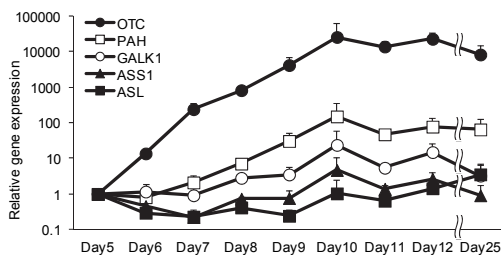
Fig. 4. Time-dependent changes of the mRNA expression of the enzymes participated in liver-specific metabolic pathways Each bar represents the mean \pm S.D. ( n = 3 , except for a part of OTC expression.).
