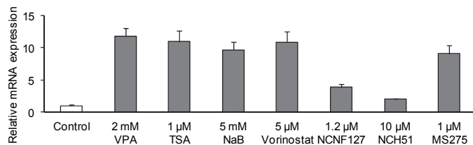
Fig. 3. ALB mRNA expression in hepatocyte-like cells differentiated with HDAC inhibitors HDAC inhibitors were added for 168 hours from day 12. Each bar represents the mean \pm S.D. ( n = 3 ). TSA, toricostatin A; NaB, sodium butyrate.
